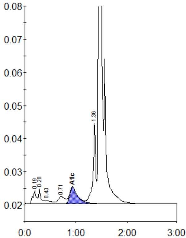
Peak table - ID: 10347616
